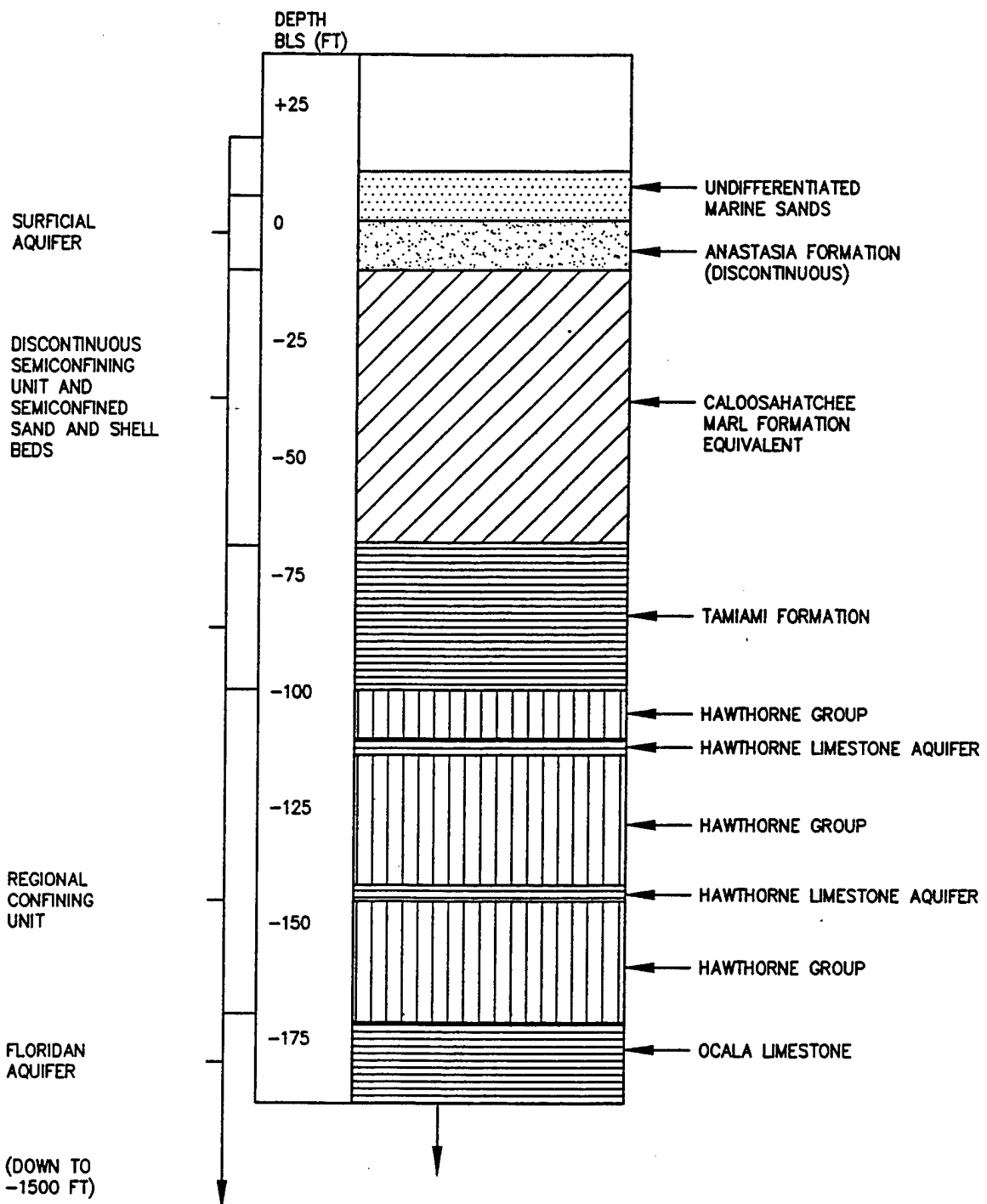
FIGURE 3.1 GENERALIZED STRATIGRAPHIC SEQUENCE Site ST-29 Intrinsic Remediation TS Patrick Air Force Base, Florida PARSONS ENGINEERING SCIENCE, INC. Denver, Colorado
