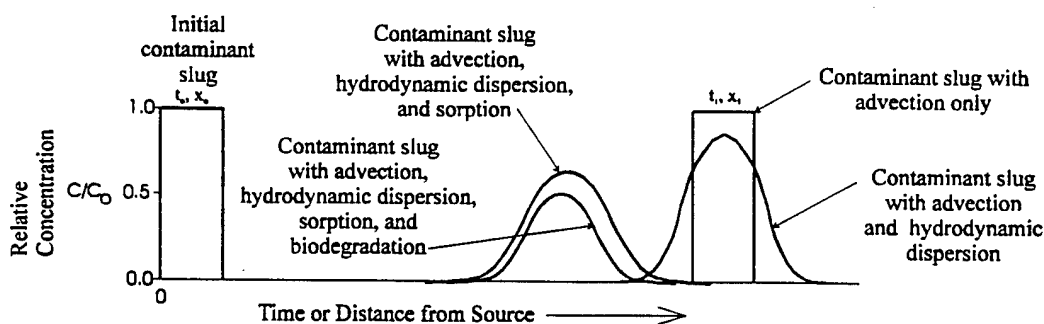
Figure B.5.2 Breakthrough curve in one dimension showing plug flow with instantaneous source resulting from advection only; the combined processes of advection and hydrodynamic dispersion; the combined processes of advection, hydrodynamic dispersion, and sorption; and the combined processes of advection, hydrodynamic dispersion, sorption, and biodegradation.
