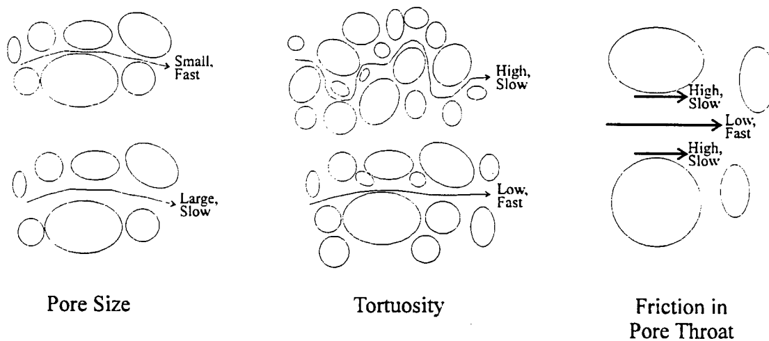
Figure B.3.1 Physical processes causing mechanical dispersion.
