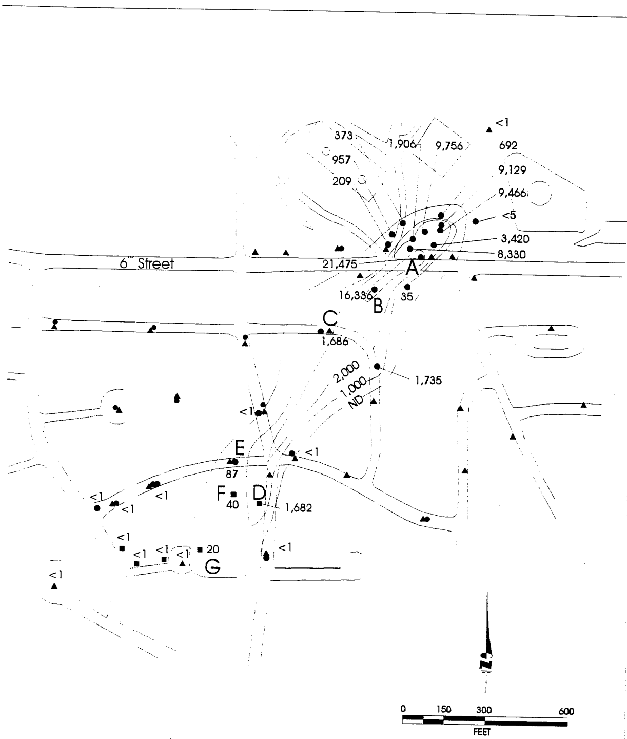
Figure C.3.5 Points Along Flow Path used for Examples C.3.7 and C.3.8
