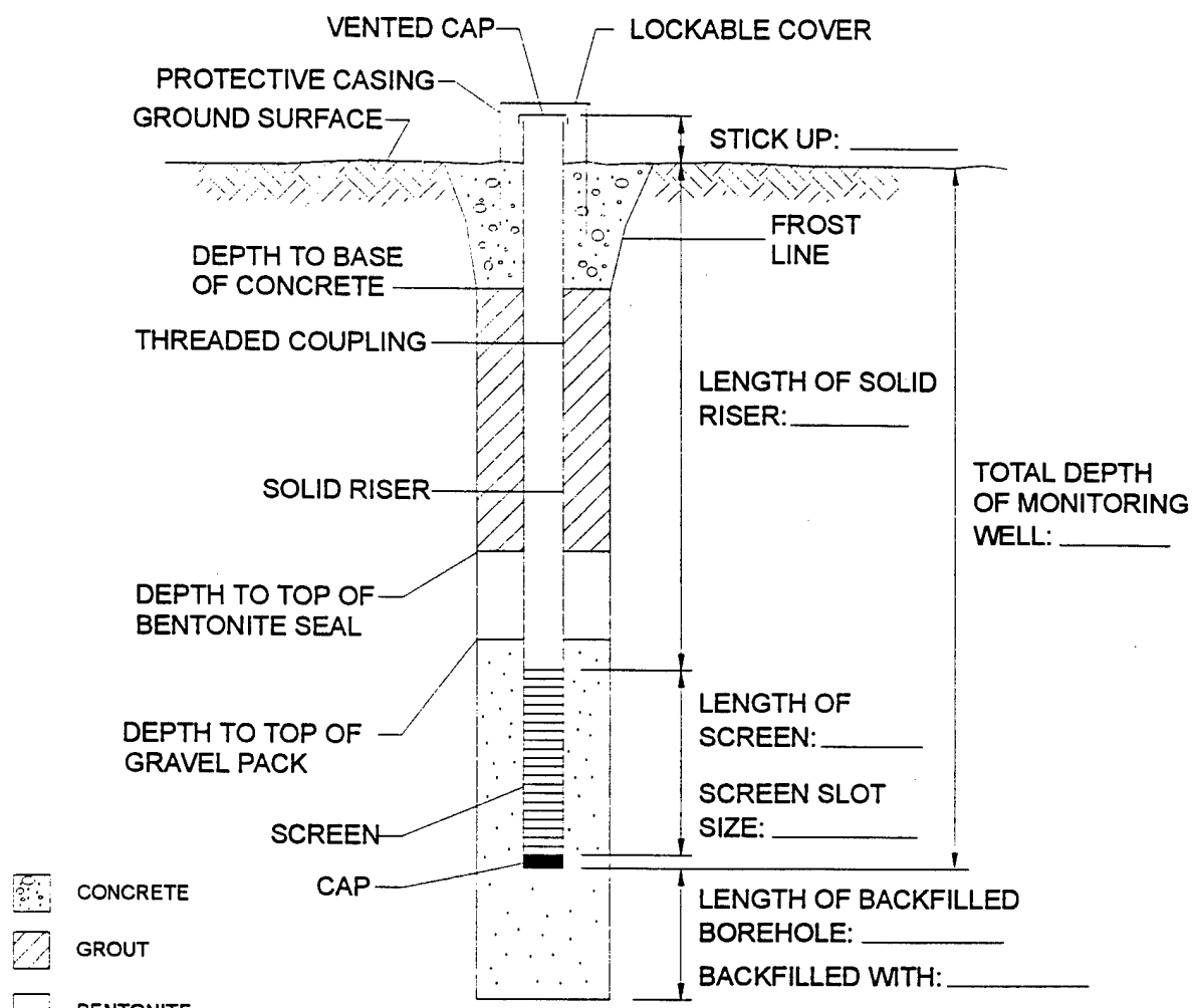
Figure A.4.1 Monitoring Well Installation Record
