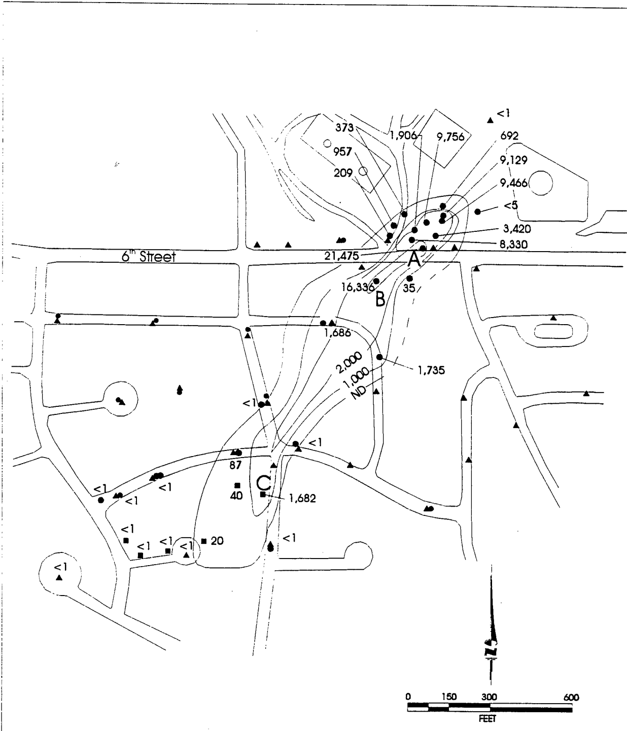
Figure C.3.4 Points Along Flow Path for Example C.3.5
