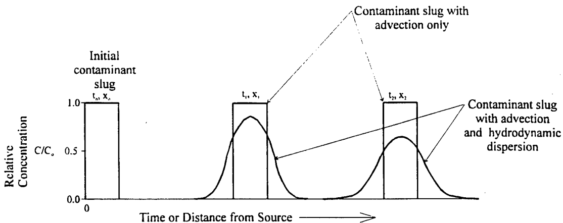
Figure B.3.3 Breakthrough curve in one dimension showing plug flow with instantaneous source resulting from advection only and the combined processes of advection and hydrodynamic dispersion.
