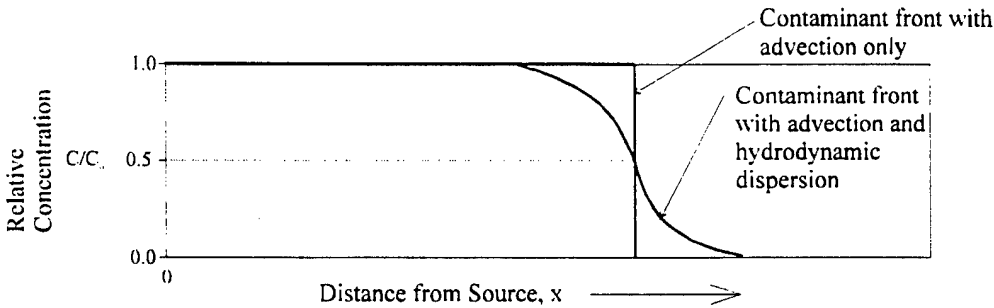
Figure B.3.2 Breakthrough curve in one dimension showing plug flow with continuous source resulting from advection only and the combined processes of advection and hydrodynamic dispersion.
